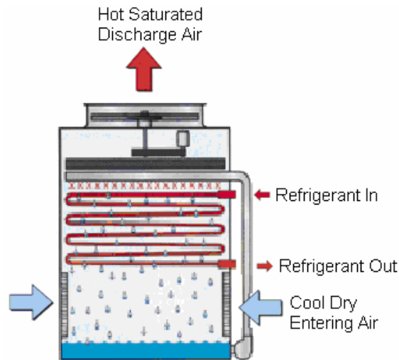
EVAPORATIVE CONDENSER
